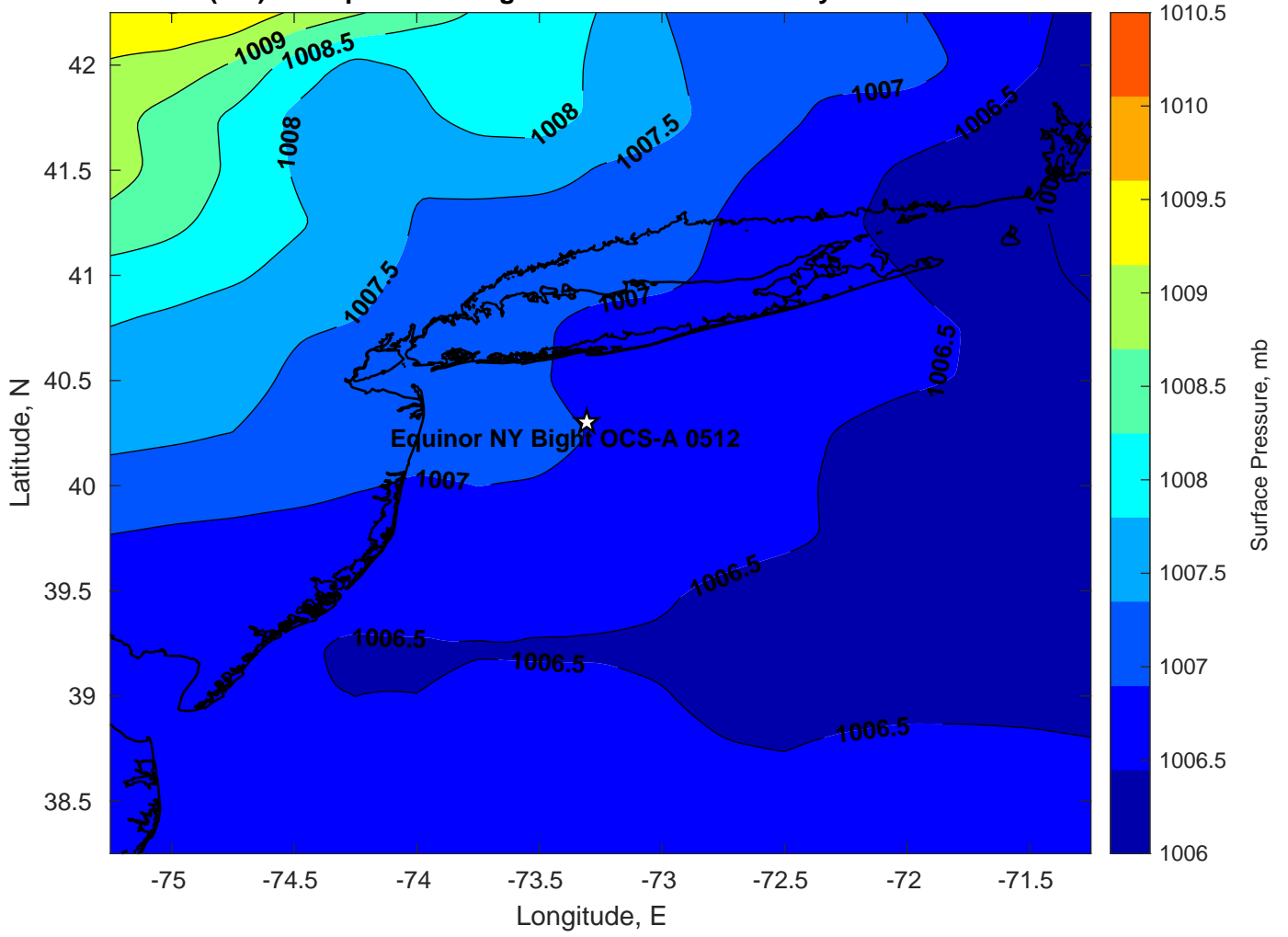
Surface Pressure (mb) for Equinor NY Bight OCS-A 0512 at 09-May-2024 12:00:00
